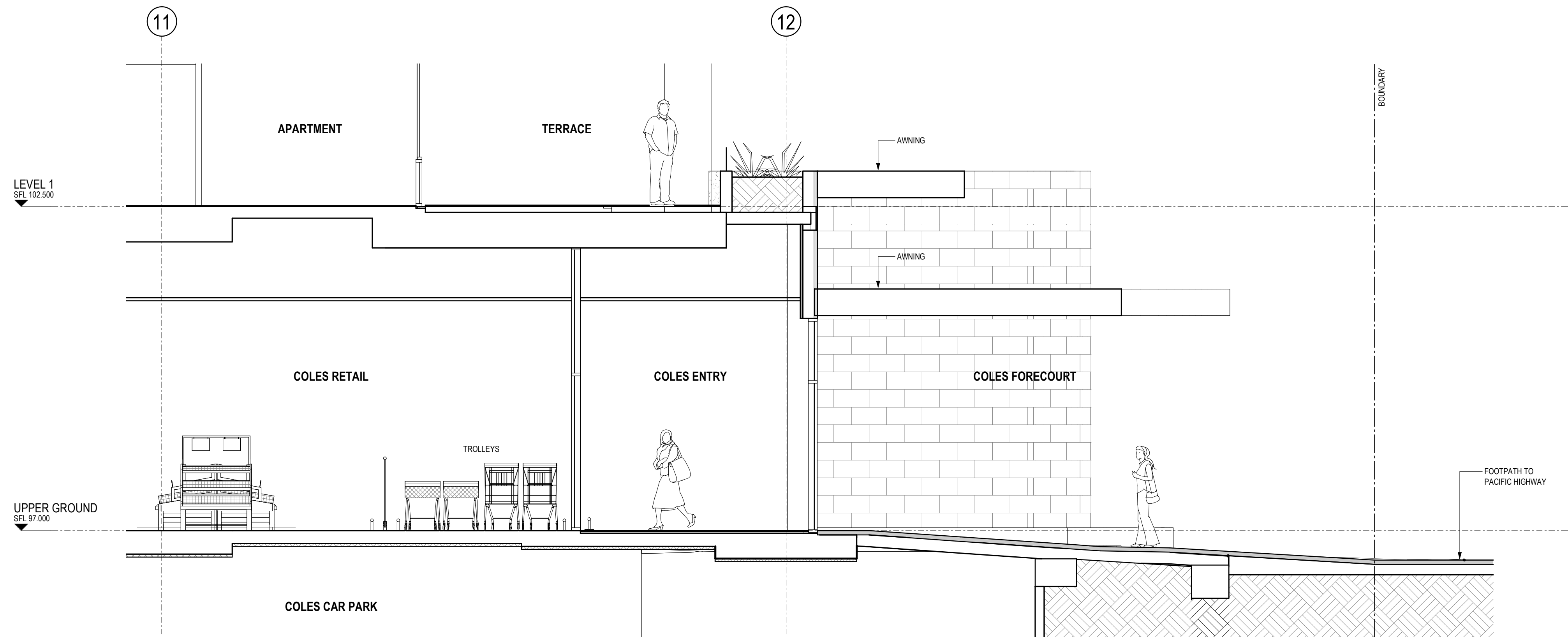
1 Coles Entry - Section at Grids D-E SCALE 1 : 50
