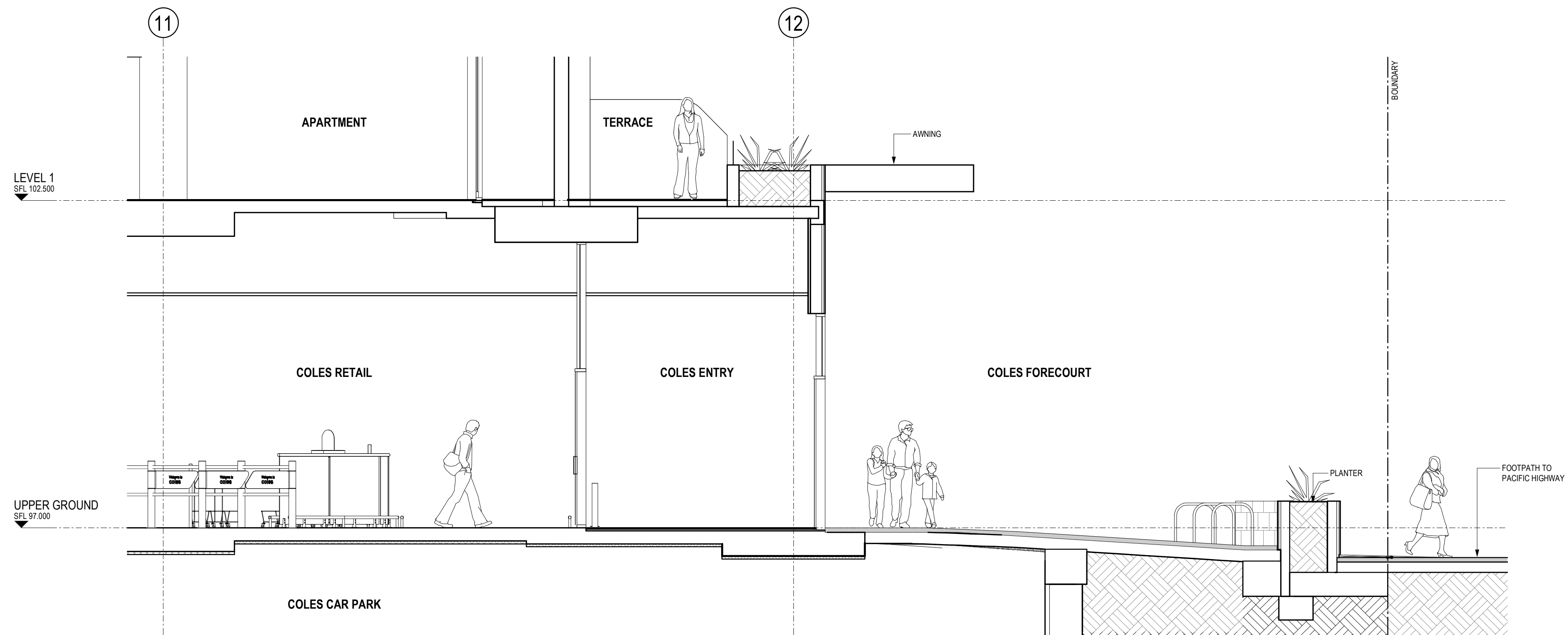
2 Coles Entry - Section at Grids E-F SCALE 1 : 50
